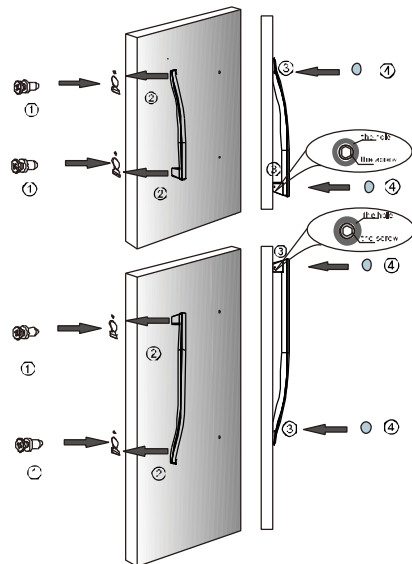
Schematic diagram of handle installation (Pictures and objects are not consistent, in order to prevail in kind)
